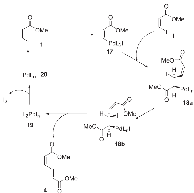
Scheme 1. Proposed mechanistic scheme for the reductive dimerisation of terminal, electron-deficient iodoalkenes exemplified by Z -iodoacrylate 1 .
